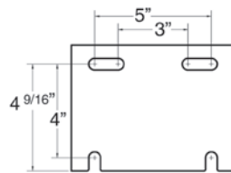
Mounting Plate
